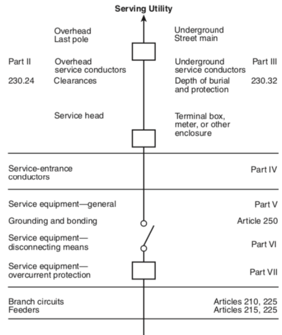
Figure 7: NEC 2017 Figure 203.1 Services © NFPA
